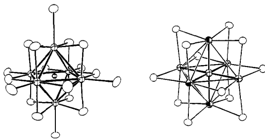
Figure 1. Zr_6X_{12} clusters with interstitial atoms. Left: the (Zr_6X_{12})X_8 unit centered by an interstitial and with the essential terminal halide atoms bound at the six metal vertices. Right: the cluster core with a better representation of the strong Zr-interstitial bonding. Halogen atoms are the open ellipsoids in both views.
