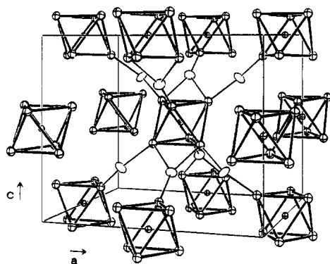
Figure 3. Zr_6Cl_{14}C : a view of the Zr_6C cluster cores and of the bridging of the central cluster by four Cl^{a-a} and two Cl^{i-a} atoms (90% probability ellipsoids).
